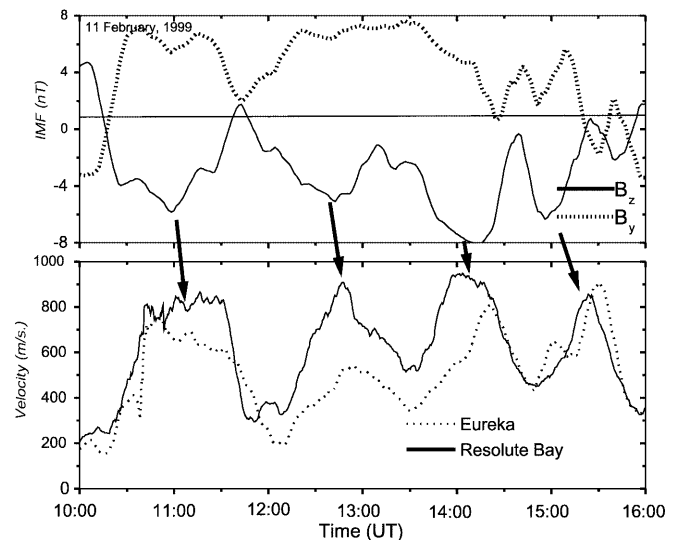
Fig. 3. Top panel: variation of IMF B_z (solid line) and B_y (dotted line). Bottom panel: convection velocity at Eureka (dotted line) and Resolute Bay (solid line) for 11 February, 1999. The convection velocity and IMF are 2½ min averages
