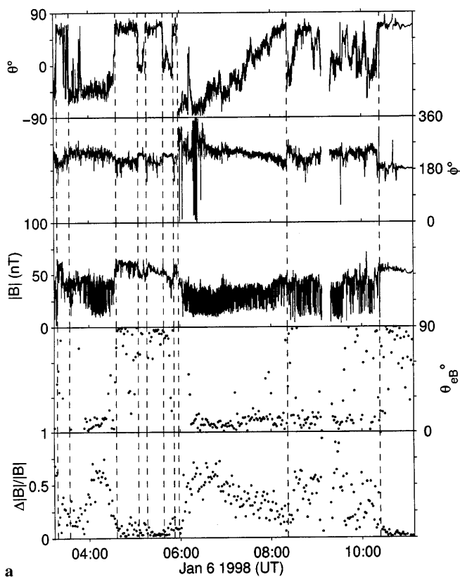
Fig. 6. a An overview of the magnetic field data recorded on January 6, 1998, in the same format as Fig. 2. The panels show field elevation ( \theta ) and longitude ( \phi ) angles in degrees, field magnitude |B| in nT, the angle between the maximum variance direction and the mean field
