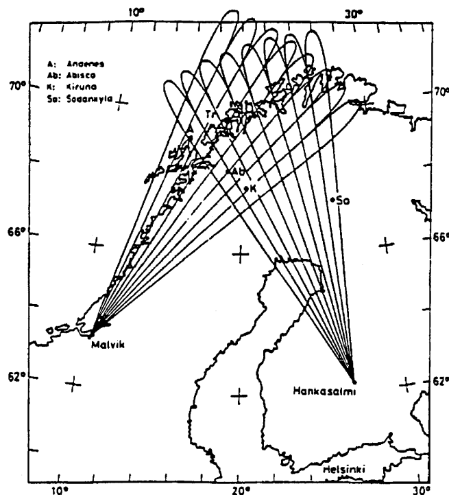
Fig. 2. Map of the two STARE radar stations and schematic representation of their radar beams. The area of overlapping beams corresponds to the field of view of the radar in which vector electric field data can be measured; from Greenwald et al. (1978)
