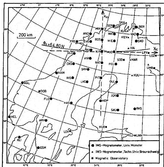
Fig. 1. Magnetometer stations of the Scandinavian Magnetometer Array (SMA); solid lines: geographical coordinates; the broken lines mark a local cartesian coordinate system that is not used in this work; from Küppers et al. (1979)
