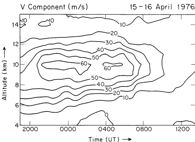
Fig. 4. Time-height cross section of the meridional wind measured by the Sunset radar on 15–16 April 1976 during the passage of a polar-front jet stream (from Green et al. , 1978)
