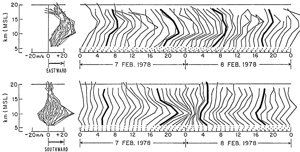
Fig. 7. Hourly-averaged wind profiles observed by the Platteville radar on 7–8 February, 1978. The velocity scale appears beneath the composite set of profiles to the left of the main panel. The time of each profile is indicated by the dotted line below each profile. Darkened profiles correspond to the times of the routine National Weather Service radiosonde ascents from Denver (from Ecklund et al. , 1979)
