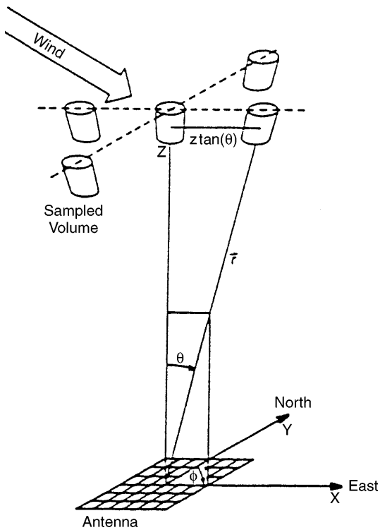
Fig. 10. Illustration of the Doppler-beam-swinging (DBS) technique for wind measurements with a five-beam radar. The altitude, range, and zenith angle are denoted by z , r , and \theta , respectively
