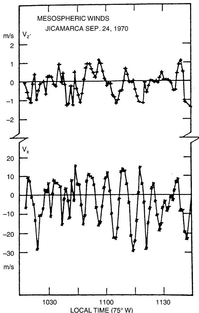
Fig. 2. Sample time series of vertical ( top ) and zonal ( bottom ) wind speeds at 85 km in the mesosphere showing large sinusoidal fluctuations due to gravity wave (from Woodman and Guillén, 1974)
