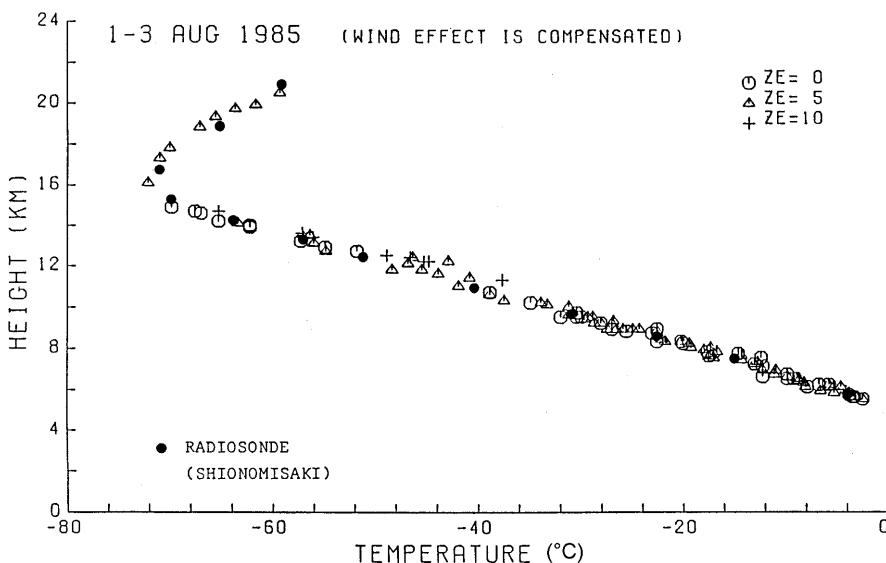
Fig. 11. Temperature profiles on 1–3 August, 1985, measured by the MU radar with RASS with three different radar zenith angles, compared with the mean temperature from routine Japan Meteorological Agency radiosonde ascents from Shionomisaki, ~157 km to the south (from Matuura et al. , 1986)
