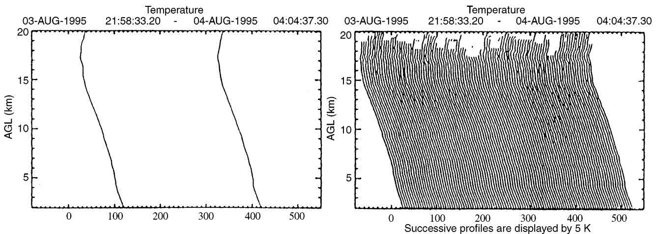
Fig. 12. (Left) temperature profiles obtained by radiosondes with an interval of six hours. (Right) temperature profiles obtained by the MU radar with RASS with an interval of 3.6 min (from Arikawa et al. , 1998)
