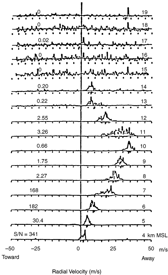
Fig. 3. Radial velocity versus altitude measured by the Sunset radar on 15 April, 1976, at 1606 105°W time, with the beam pointed at 30° to the north (from Van Zandt et al. , 1978)
