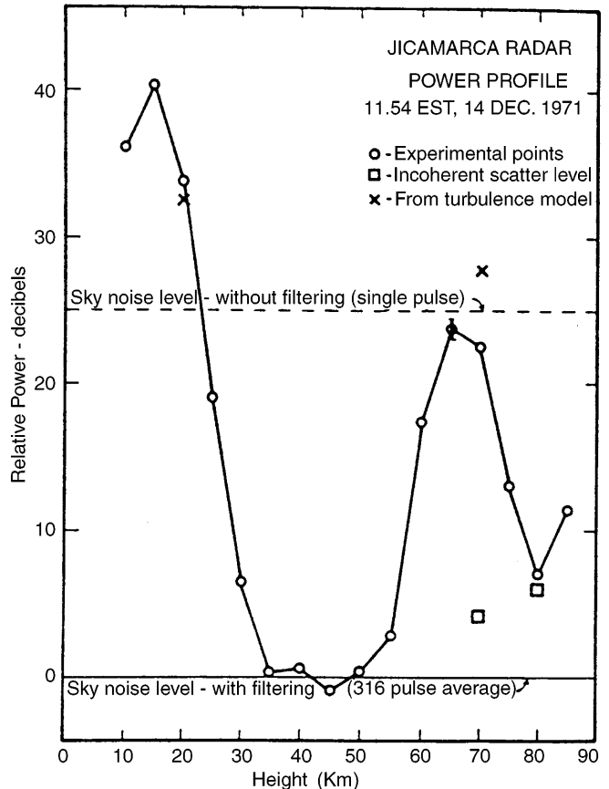
Fig. 5. Backscattered power profile observed by the 50 MHz Jicamarca radar (from Woodman and Guillén, 1974)
