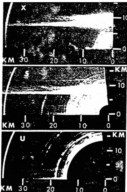
Fig. 1. RHI (range-height-intensity) scans at 3.2 cm (X band), 10.7 cm (S band), and 71.5 cm (UHF band) wavelengths (top, center, and bottom panels, respectively) at 90° azimuth taken at 1030 EST 18 February 1966 at Wallops Island, Virginia. The layer at 12 km in the bottom panel was visible on the original photographs (from Atlas et al. , 1966b)
