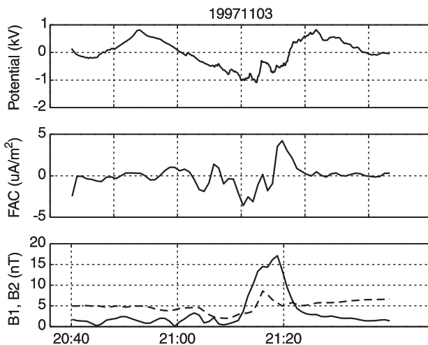
Fig. 6. Event 971103 21:05–21:25 UT. B_2 is smaller than B_1 so the FAC estimate is rather reliable. The potential and the FAC have the same sign so this event could support the upward extended U-shaped potential picture, but the magnitude of the potential ( \sim 1 kV) is small. Among our 78 events only two are somehow compatible with the upward extended U-shaped potential picture, and this is one of them
