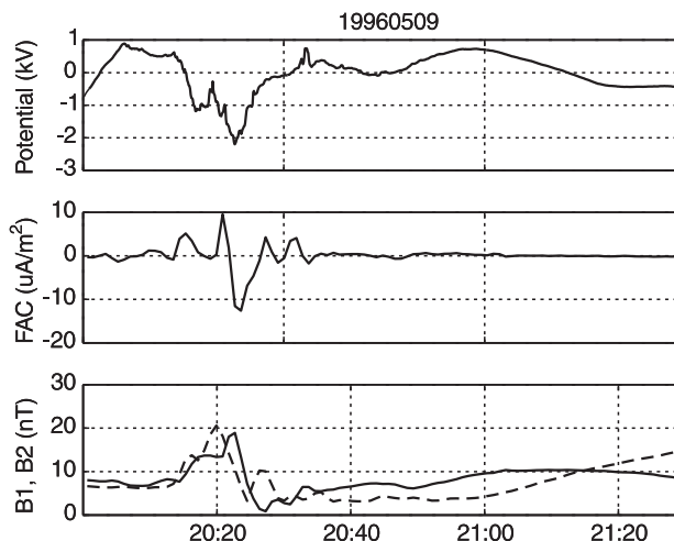
Fig. 5. Event 960509 20:15–20:30 UT. Since B_2 \sim B_1 , the FAC is not very reliable. As the potential and the FAC are both negative, this could support the upward extended U-shaped potential, but the magnitude of the potential is not very large. Among our 78 events this is one of the two that are somewhat compatible with the upward extended U-shaped potential picture
