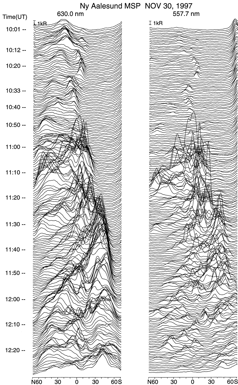
Fig. 2. Meridian scanning photometer (MSP) plots of auroral observations from Ny Alesund (at 630.0 and 557.7 nm) during the interval 1000–1230 UT on November 30, 1997
