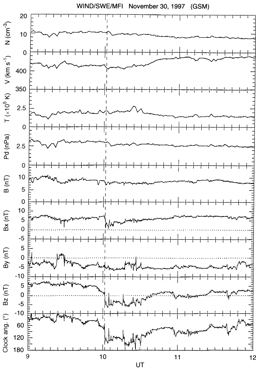
Fig. 1. Solar wind plasma and IMF observations from Wind on November 30, 1997. Shown from top to bottom are proton density (in \text{cm}^{-3} ), bulk speed (in \text{km/s} ), proton temperature (in K), dynamic pressure (in nPa), the magnetic field magnitude and components B_x , B_y , and B_z (in nT) and the IMF clock angle (degree). The southward turning of the IMF at 1000 UT is marked by a vertical line
