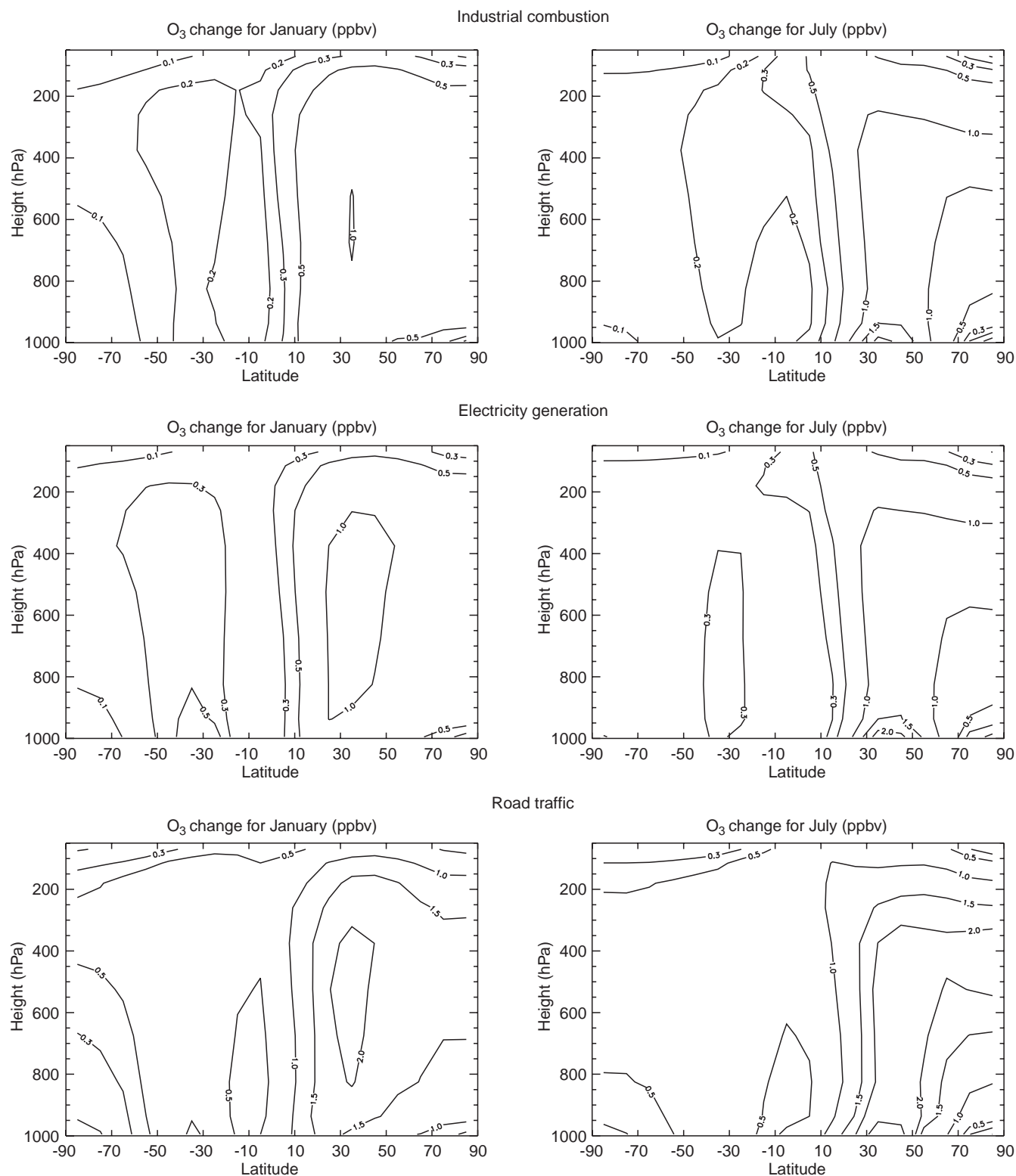
Fig. 7. Contribution of the NO x emissions from industrial combustion, electricity generation and road traffic to the zonally-averaged ozone concentrations for the year 1990 (the changes in the
