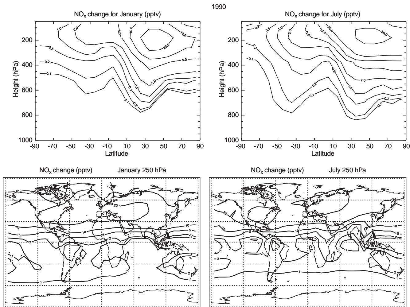
Fig. 3. \text{NO}_x perturbation for January and July due to aircraft emissions for the reference year 1990. Top shows the zonally-averaged \text{NO}_x perturbation (pptv). The lower panels show the distribution of the \text{NO}_x perturbation at 250 hPa (pptv)
