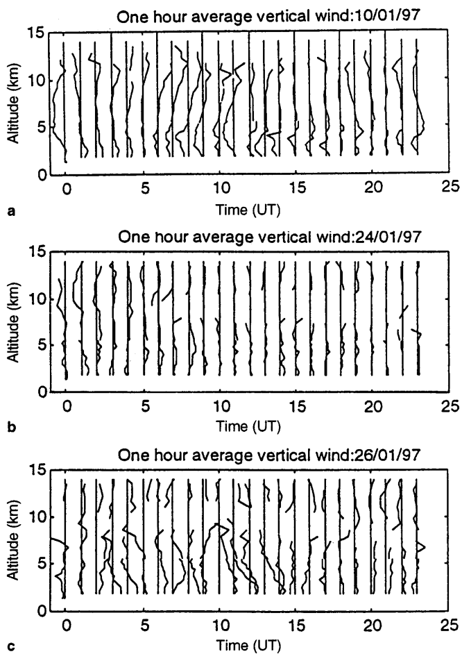
Fig. 8. Profiles of hourly vertical wind averages for 10 January 1997 (a), for 24 January 1997 (b) and for 26 January 1997 (c). The distance between the profiles corresponds to 1 m/s
