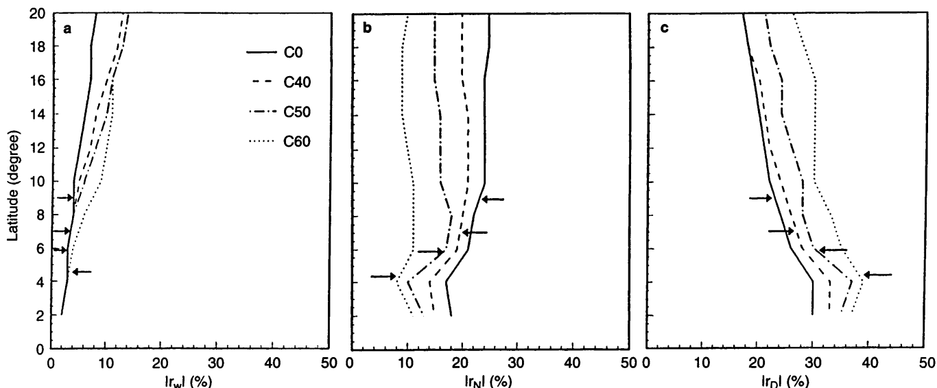
Fig. 5a–c. Linear energy flux coefficient (%) at different latitudes (°). (a) r_W , (b) r_{Nl} and (c) r_{Dl} . Solid line for C0. Dashed line for C40. Center-dashed line for C50. Dotted line for C60. The arrows indicate the critical latitude values for the investigated boundaries. T = 60 days
