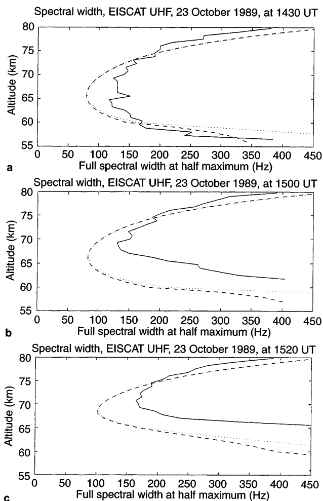
Fig. 6a–c. Observed spectral widths as functions of height ( solid lines ), and model results for full plasma calculation ( dashed lines ) and collisional approximation ( dotted lines ). a For 1430 UT, b for 1500 UT, and c for 1520 UT. See text for zenith angle dependence of the assumed photodetachment and photodissociation rates
