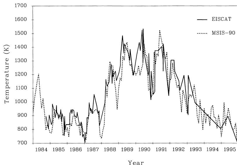
Fig. 1. Variation of the unperturbed ion temperature, derived from the EISCAT CP-1 and CP-2 observations at 312 km altitude ( solid line ). The dotted line indicates the variation of the thermospheric temperature at the same altitude, from the MSIS-90 model
