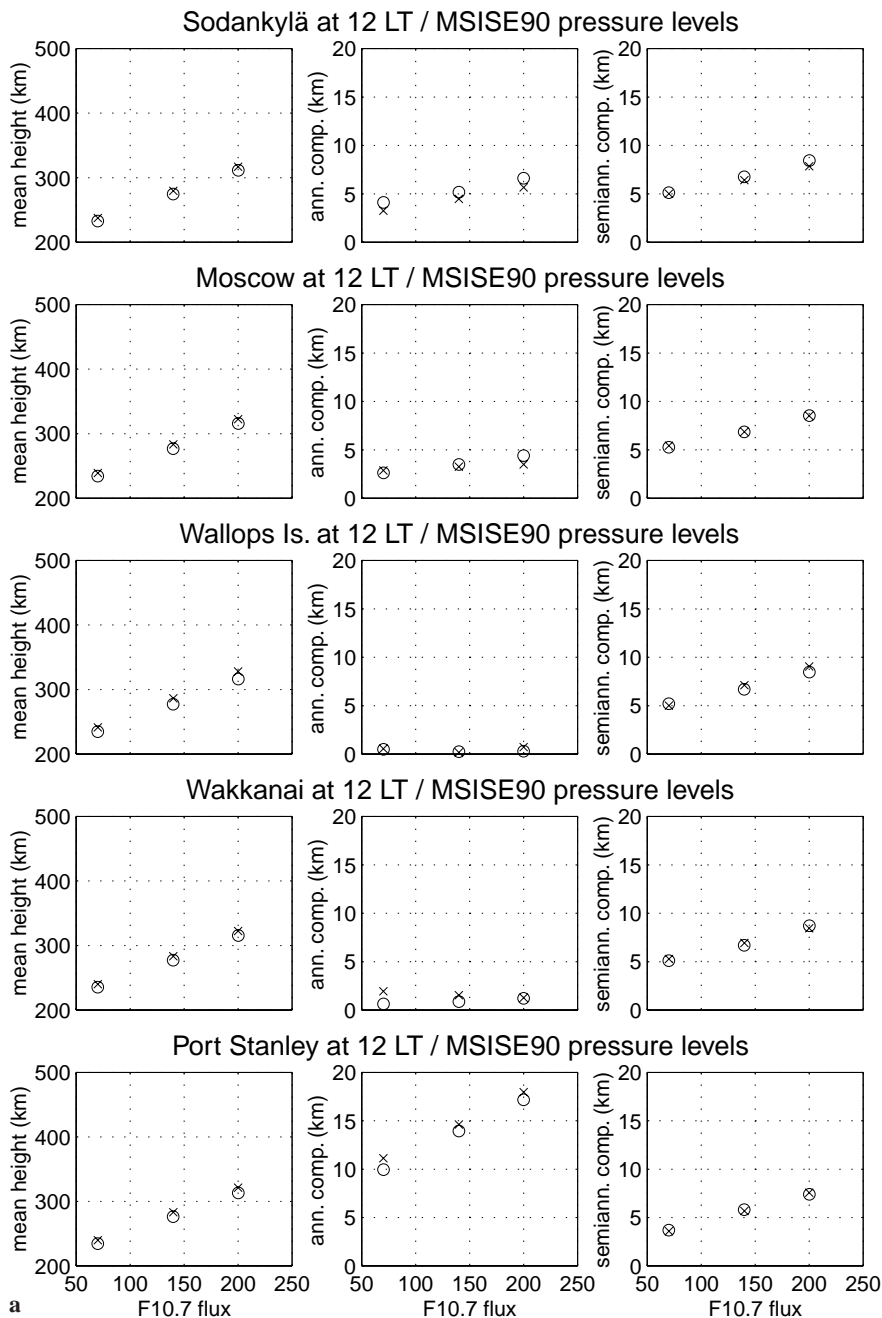
Fig. 7. a Annual means, annual and semi-annual amplitudes of the fixed pressure-level 20 \mu\text{Pa} (approximately corresponding to daytime h_m\text{F}2 ) plotted versus 10.7 cm solar flux at five stations for noon (12 LT). b Annual means, annual and semiannual amplitudes of the fixed pressure-level 2 \mu\text{Pa} (approximately corresponding to nighttime h_m\text{F}2 ) plotted versus 10.7 cm solar flux at five stations for night (02 LT)
