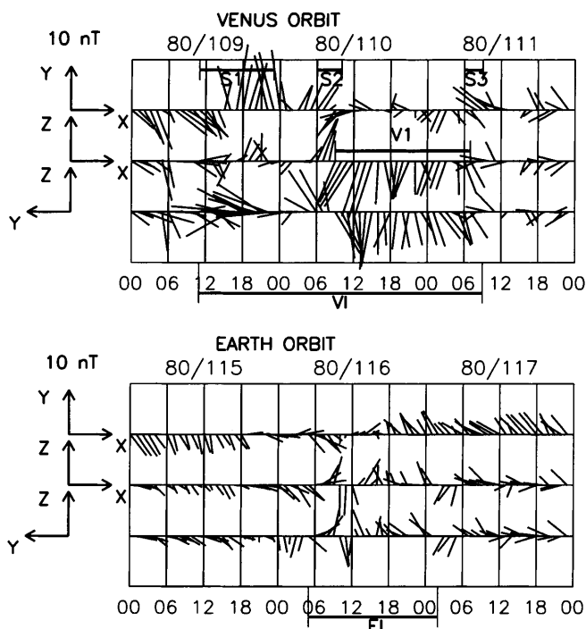
Fig. 5. IMF vector plots for sector boundary pair of no. 5 in Table 1. A multiple current sheets crossing is observed at Venus ( upper panel ), while a single current sheet is observed at Earth ( lower panel )
