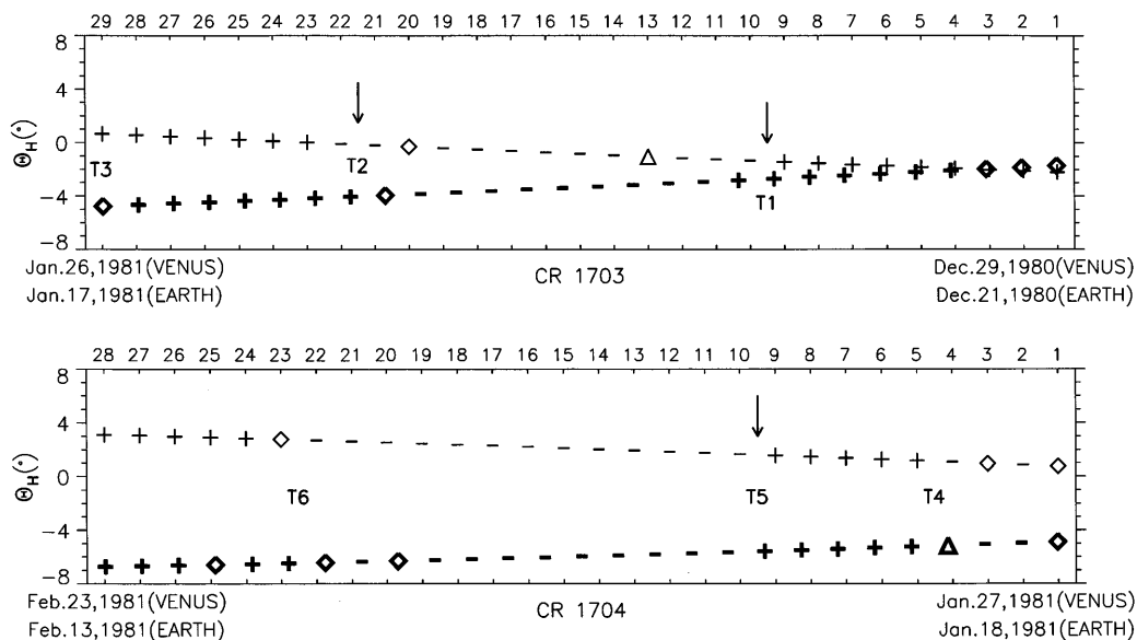
Fig. 1. Daily averages of the IMF polarity observed at Venus ( thin ) and Earth ( thick ) for Carrington rotation (CR) 1703 ( upper panel ) and 1704 ( lower panel ), adjusted for the 4-day and 5-day transit times of
