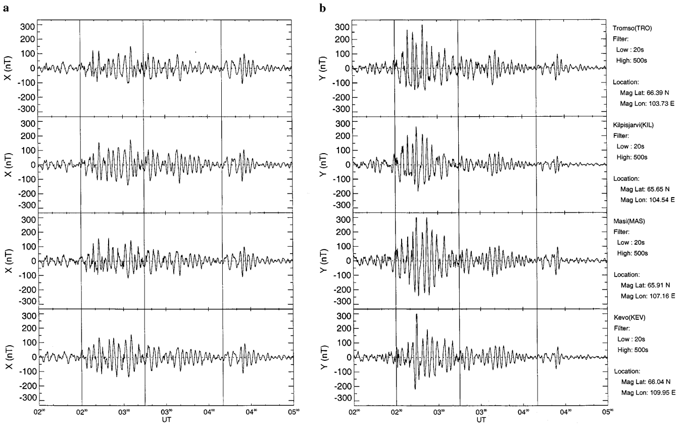
Fig. 1a, b. Band-pass filtered magnetometer data between 0200 and 0500 UT from Tromso (TRO), Kilpisjarvi (KIL), Masi (MAS) and Kevo (KEV). The filter bandwidth is 20 to 500 s. The X components
