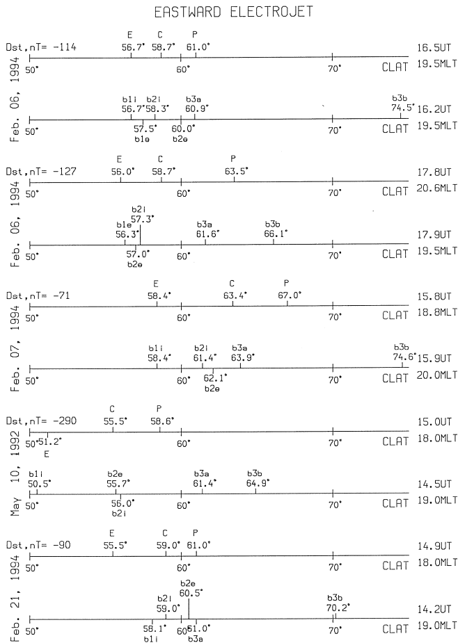
Fig. 5. The center (C) and boundaries (E, equatorial and P, polar) of eastward electrojets in the course of magnetic storms on February 06–07, February 21, 1994 and May 10, 1992 in the evening sector. For DMSP F08 and DMSP F10 passes with UT and MLT crossing close to electrojets the location of plasma domain boundaries according to Newell et al. (1996) is presented: b1e, i , are boundaries of “zero – energy”, usually determined by the softness channels; b2e are points where electron average energy is neither increasing nor decreasing with latitude; b2i is precipitating ion energy flux maximum; b3a is the most equatorward electron acceleration event identified, equatorial boundary of the structural auroral forms; b3b is the most poleward such event, polar boundary of the discrete auroral forms. Hourly mean Dst values correspond to UT of passes
