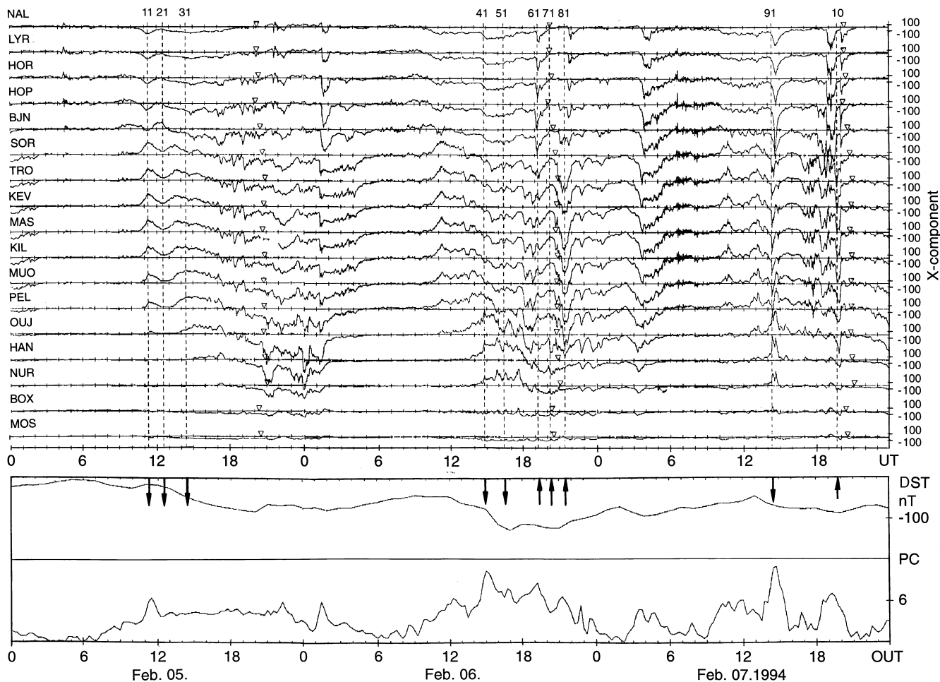
Fig. 1. Variations of the magnetic field X component along the IMAGE chain during storm main phase on February 05–07, 1994 (top). Dotted lines (vertical) correspond to 10 UTs with latitudinal cross sections of the \Delta X and \Delta Z components presented further in the text. The Dst and the PC indices of the magnetic field
