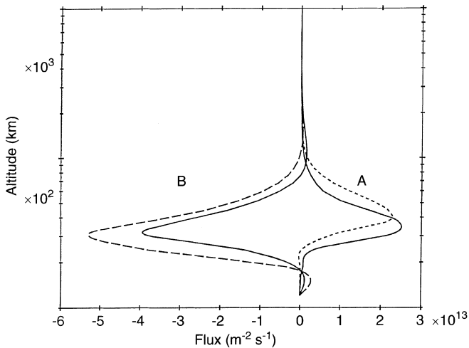
Fig. 5. Model O^+ flux values during the enhanced velocity event at 9:23 UT (---), point A on path, and at 9:53 UT (- - -), point B on the path. Fluxes at these points with no enhanced velocity are shown for comparison (—), Positive flux is upwards, negative values represent downward fluxes
