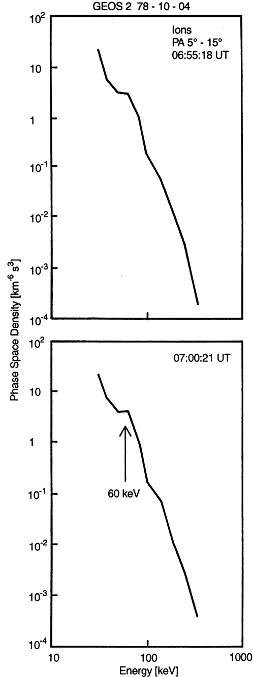
Fig. 7. Phase space density of energetic protons recorded onboard GEOS-2 in the pitch-angle range 5^{\circ} – 15^{\circ} on October 4, 1978, 0655:18 and 0700:21 UT
