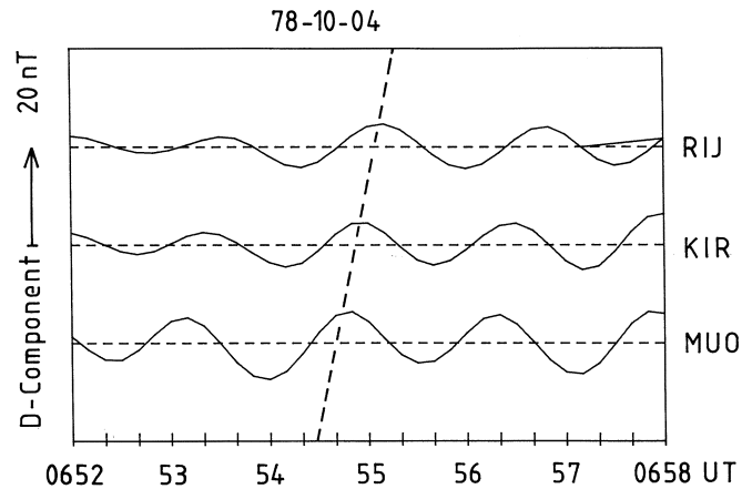
Fig. 3. Magnetic field variations recorded along the three east-west aligned stations RIJ, KIR, and MUO. Geomagnetic latitude of the three stations is 64.8^\circ \pm 1^\circ . The dashed line connects corresponding maxima at the different stations
