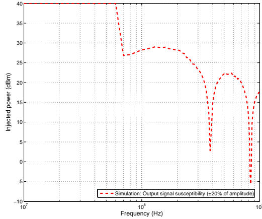
Fig. 16. Immunity simulation without the directional coupler
