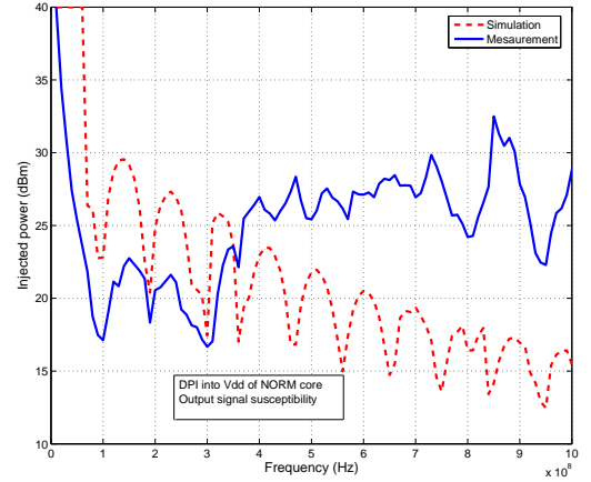
Fig. 18. Immunity simulation (dashed line) and measurement (solid line) for the lossless DPI model
