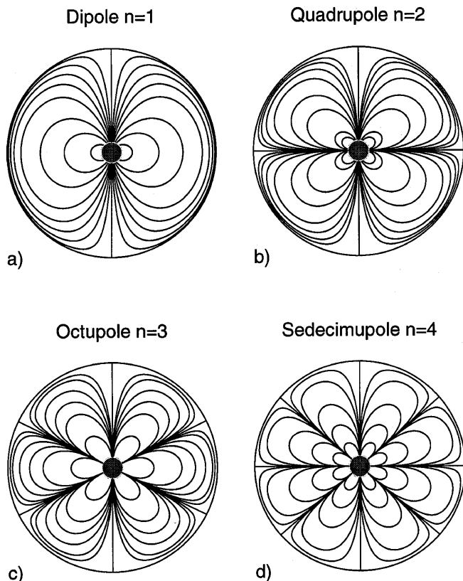
Fig. 2a–d. Illustrative magnetic-field-line configurations for low-degree zonal (axisymmetric) magnetic multipoles ( m = 0 ): a dipole ( n = 1 ), b quadrupole ( n = 2 ), c octupole ( n = 3 ), and d sedecimupole ( n = 4 ). In this illustrative figure (and in Figs. 3 and 4), the radius of the magnetopause is taken to be ten times the radius of the Earth ( R_M = 10R_E )
