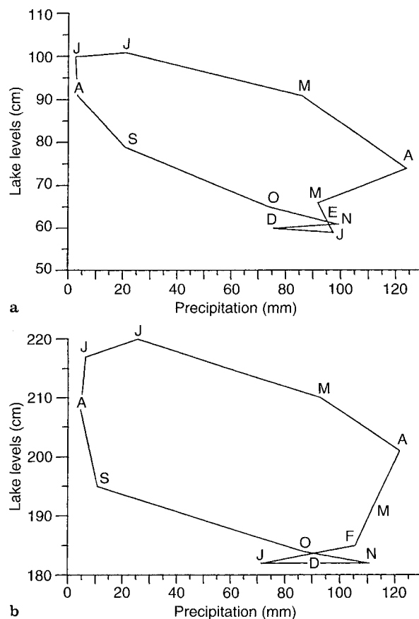
Fig. 7a, b. Lake level-Tatvan precipitation polygon a 1944–1968 period, b 1969–1994 period
