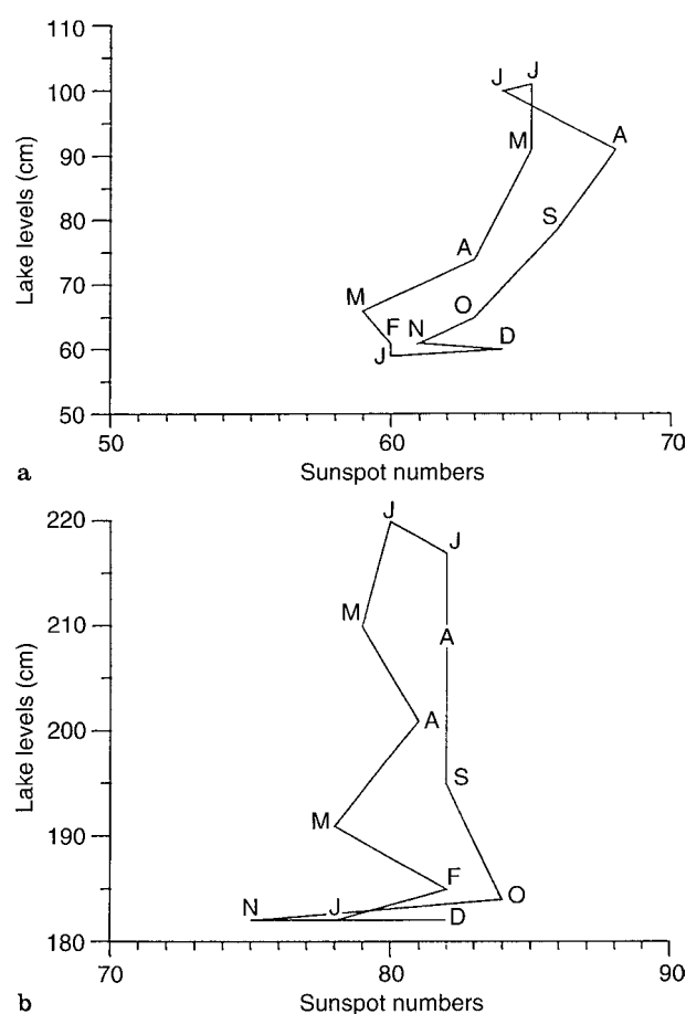
Fig. 9a, b. Lake level-sun spot number polygons a 1944–1968 period, b 1969–1994 period
