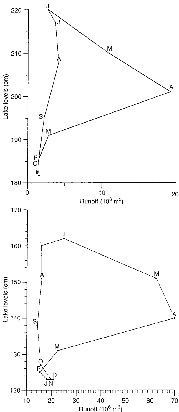
Fig. 10a, b. Lake level-local runoff polygons a Süfrezor, b Bendimahı
