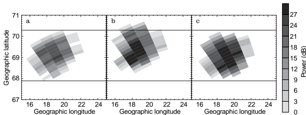
Fig. 10a–c. CUTLASS Finland spatial plots for 22 April 1996. a 1447 UT, heater beam at -13^\circ to the vertical. b 1504 UT, heater beam pointing vertically. c 1534 UT, heater beam at -13^\circ to the vertical. Horizontal lines are drawn at 67.9^\circ and 70.3^\circ latitude
