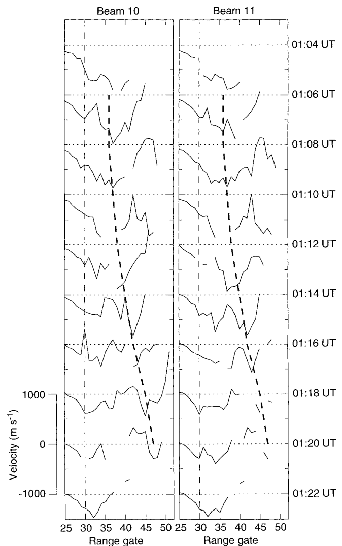
Fig. 5. Stack plots of line-of-sight backscatter velocity as a function of range gate of beams 10 and 11 between 0104 UT and 0122 UT. Range gates 25 and 50 correspond to approximately 68^\circ\text{N} GMLAT and 79^\circ\text{N} GMLAT. The vertical dashed line indicates the demarcation of zonal and meridional flow at 72^\circ\text{N} . A poleward-progressing velocity enhancement is observed, the thick dashed line being a fit-by-eye to this poleward motion
