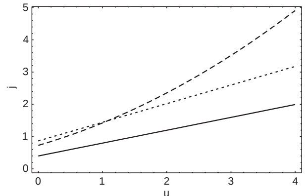
Fig. 9. Comparison of current-voltage relationships in kinetic theory (solid; Eq. 38), fluid theory with \gamma = 3 (dotted; Eq. 56) and fluid theory with \gamma = 5/3 (dashed; Eq. 55)
