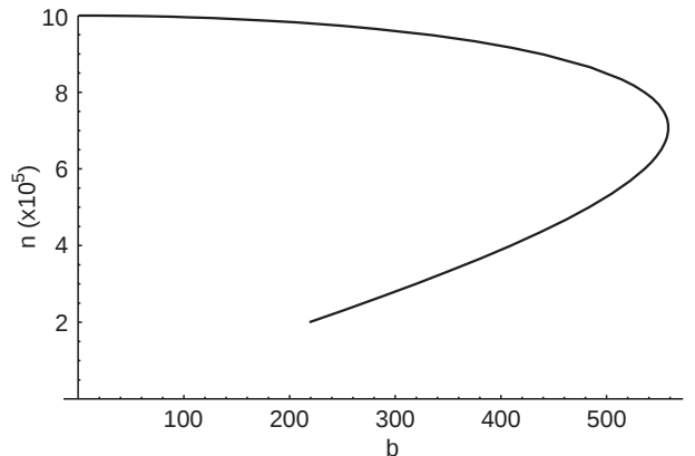
Fig. 10. Behavior of Eq. (80)
