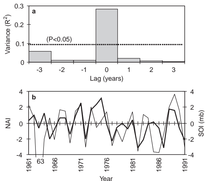
Fig. 2. a Results of a lag correlation analysis (omitting data for 1963 and 1989) showing the variance in the mean annual SOI explained by the NAI, when the latter index led or lagged the SOI by up to 3 years; b Superimposed time series of the NAI (light line) (the 1963 value of -12 being off scale), and the mean annual SOI (heavy line)
