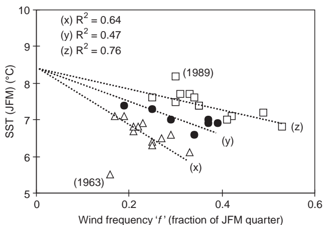
Fig. 1. Relationships between SST and W-NW-N (240 °–30 °) wind frequency ( f ) during the first quarter (JFM) of each calendar year between 1961 and 1991. Data for the exceptionally cold winter of 1963, when anticyclonic blocking conditions prevailed over the NA (Barry and Chorley, 1992), and for the exceptionally warm winter 1989, when an anomalous poleward displacement of the Gulf stream took place (Ginkul and Gavriluk, 1991), were not included in the regression analyses. The regression relationships were forced through a common intercept (8.4 °C) in keeping with their divergent tendency
