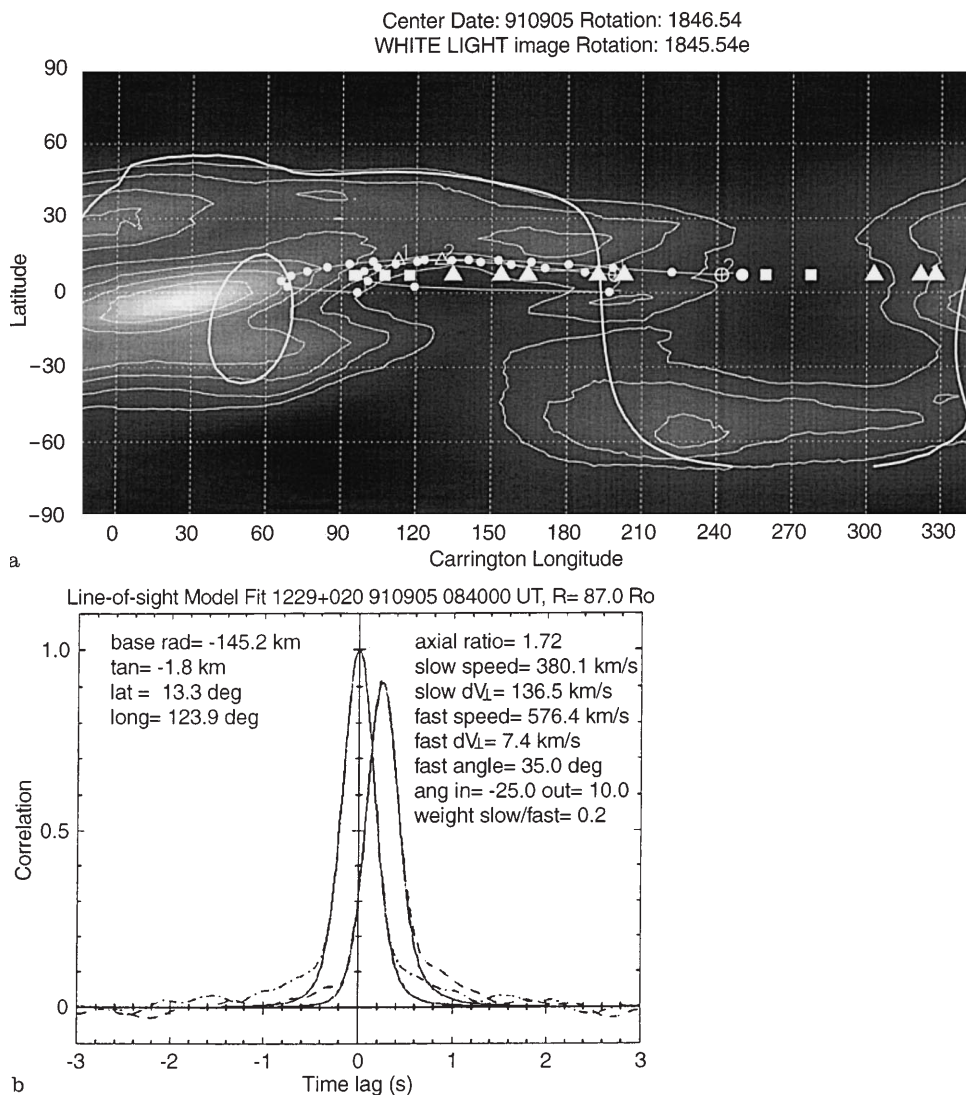
Fig. 8. a White-light map showing the ray-path for an EISCAT observation of 1229+020 on 5 September 1991, projected down to 1.7 R with assumed velocities of 750 \text{ km s}^{-1} (line 1) and 325 \text{ km s}^{-1} (line 2). The white line stretching across the whole of the map is the magnetic equator of the Sun, calculated from Stanford magnetic data. The white triangles mark regions of intermediate-velocity flow, measured by the IMP-8 spacecraft at 215 R as the region observed
