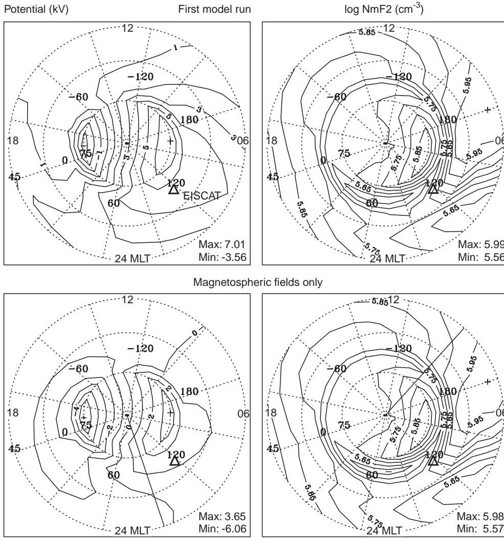
Fig. 4. Potential distributions (left panels) and isolines of \log(\text{NmF2}) per \text{cm}^{-3} (right) for the first model run. The upper panels illustrate the version with magnetospheric and dynamo electric fields while the bottom panels illustrate the version with the action of magnetospheric electric fields only. The polar plots show the northern hemisphere distributions at 00 UT with magnetic local time and magnetic latitude (down to 45^\circ ) as coordinates. The EISCAT station location is indicated by a thick triangle
