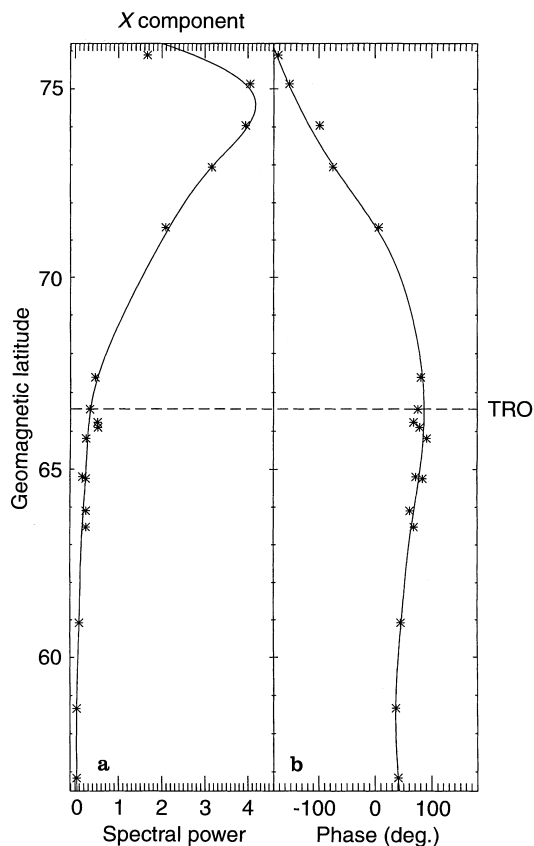
Fig. 6a, b. Latitudinal a Fourier spectral power and b phase profiles of the 4 mHz spectral component derived from the X -component magnetometer data illustrated in Fig. 5. The dashed line indicates the location of the Tromsø (TRO) magnetometer
