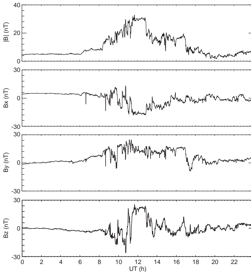
Fig. 3. The magnitude and components of the IMF measured by the WIND satellite on 27 November 1995 (day-number 331)
