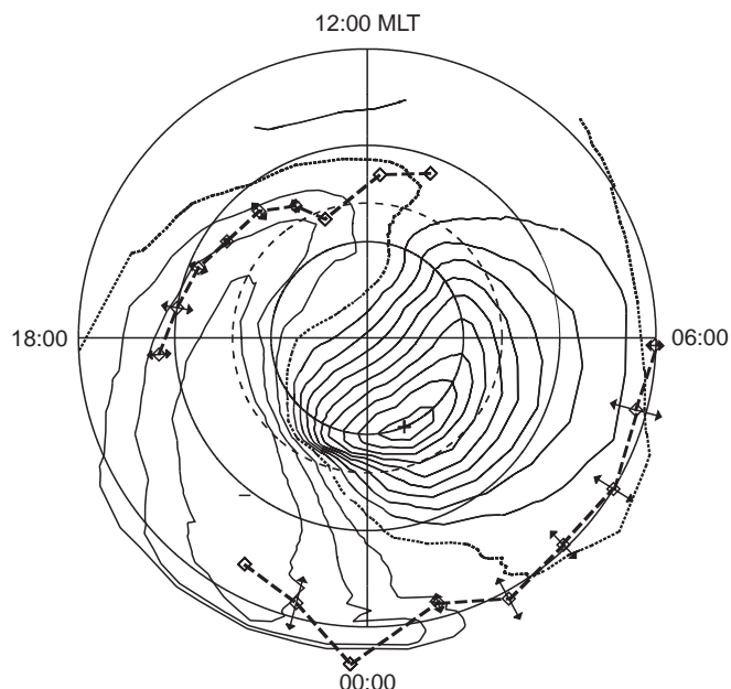
Fig. 6. Dial plot showing the average position of the postmidnight mid-latitude trough and the dayside trough during the quiet geomagnetic conditions as a function of corrected geomagnetic latitude ( 60\text{--}90^\circ\text{CGM} ) and MLT. The squares indicate the location of the trough minimum and the arrows the associated standard deviation. Superimposed is the IZMEM electric potential contours at 5-kV intervals for the mean IMF of the quiet period
