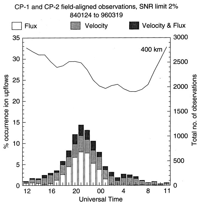
Fig. 8. Diurnal distribution of upflows (400 km) simultaneous with either an enhanced ion or electron temperature
