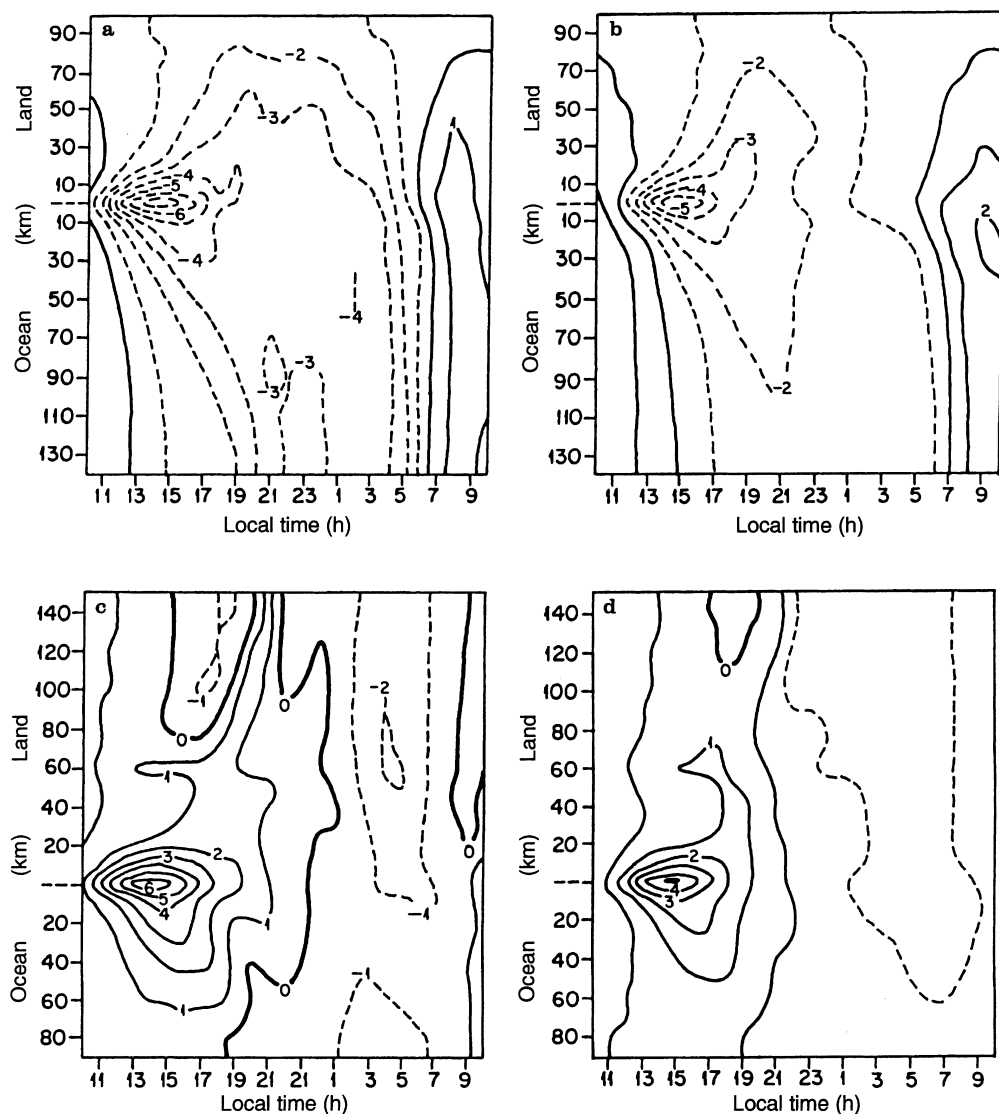
Fig. 6a–d. Simulated temporal variation of the horizontal extension of the sea-breeze at the 990 hPa level: a EW variation of the u-component along line AB (Fig. 1) simulated for OND. The easterlies are indicated by broken lines ; and the westerlies are represented by solid lines ; b as a , except for AMJ; c SN variation of the v-component along line CD simulated for OND. The southerlies are indicated by solid lines and the northerlies are represented by a broken line ; and d as c , except for AMJ. Units are \text{m s}^{-1}
