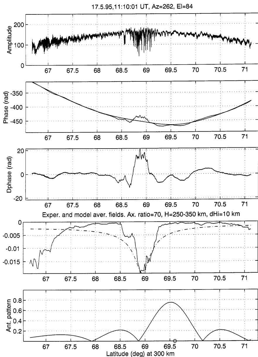
Fig. 2. Same as Fig. 1, but for the satellite pass during the operation of the heating facility. The bottom panel shows the spatial cross section of the calculated antenna pattern of the Tromsø facility as a function |\sin x / x| using the satellite geometry and the parameters of array 2. The open circle on the x-axis indicates the latitude of the heating facility
