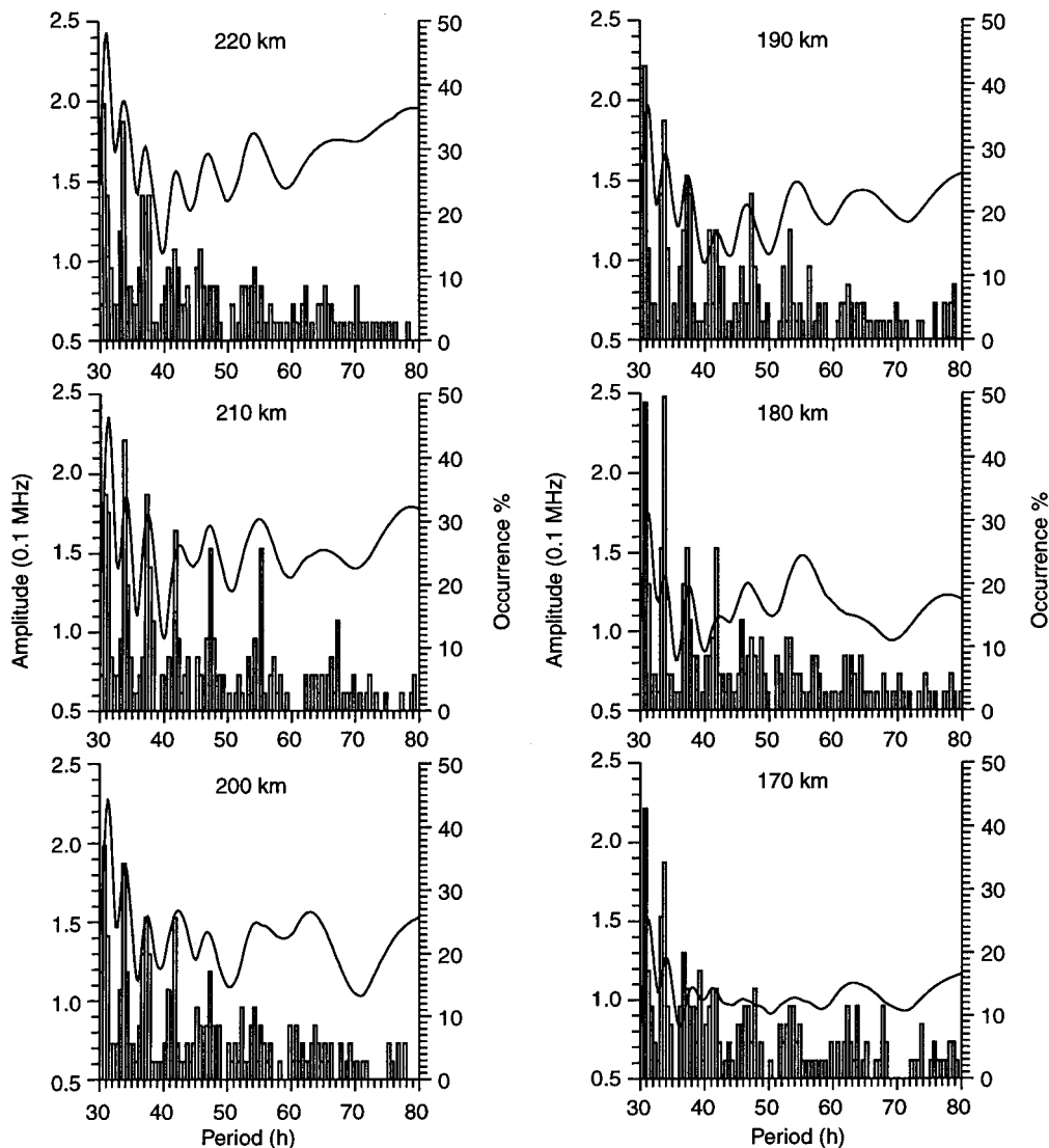
Fig. 2. Averaged amplitude spectra ( solid line ) and percent-age occurrence of periods ( histograms ) of ionospheric plasma frequency variations during 1995. The left y-axis represents the averaged amplitude and the right y-axis the percentage occurrence
