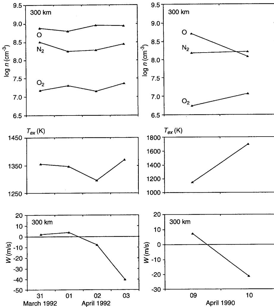
Fig. 5. Calculated neutral composition (at 300 km) and exospheric temperature T_{ex} (top and middle panels) and calculated vertical plasma drift (bottom panel) for 31 March–3 April 1992 (left) and 09–10 April 1990 (right)
