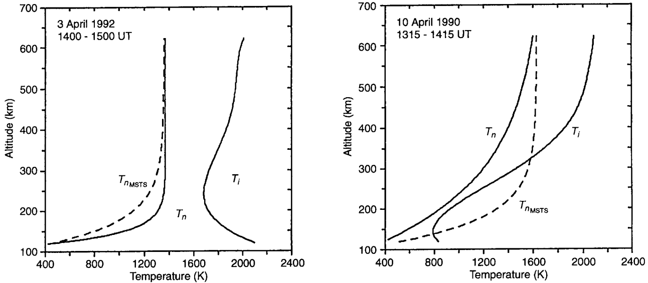
Fig. 6. Calculated and MSIS-83 T_n(h) profiles together with the observed T_i(h) profile for the disturbed days 3 April 1992 (left) and 10 April 1990 (right)
