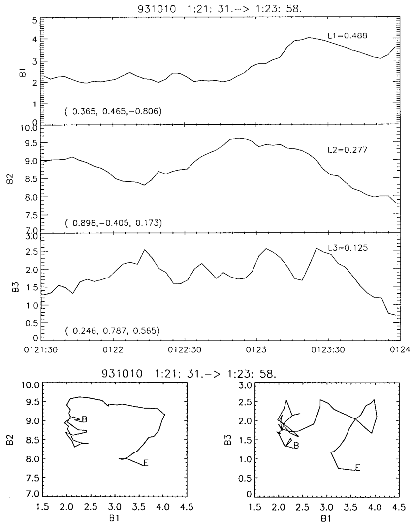
Fig. 7. 3 s averages of the GEOTAIL magnetic field data across the boundary layer plasmoid displayed in principal axis coordinates. Hodograms of the field variation in two orthogonal planes are shown in the bottom panels
