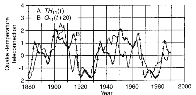
Fig. 13. Quake-temperature teleconnection
