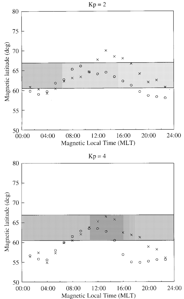
Fig. 6. The upper panel depicts the DMSP ion (circles) and electron (crosses) boundaries with respect to the SABRE field of view (illustrated by the shaded region) determined for a K_p value of 2. The lower panel depicts the boundary locations for a K_p value of 4. The regions in which the ion and electron boundaries substantially separate (i.e. 1200 MLT to 2000 MLT) coincides with the MLT sector in which SARAS are predominately observed
