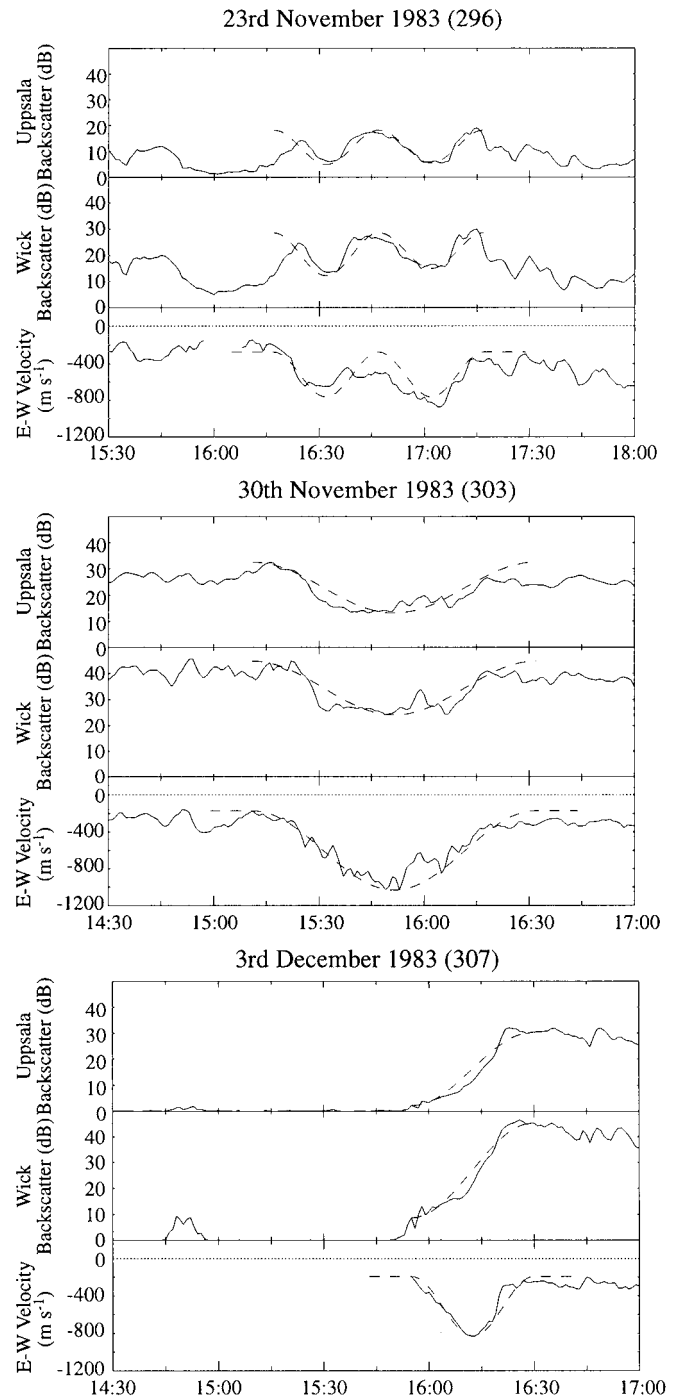
Fig. 3. Three examples of the backscatter intensity and east-west velocity variations during SARAS events. The dotted line in each panel depicts the function form of the idealised function employed by the selection algorithm to locate the events
