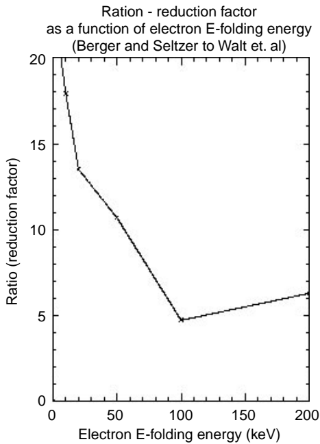
Fig. 7. The reduction factor for calculating the X-rays emitted at 135^\circ , nadir angle (Walt et al. , 1979) from the X-rays emitted into the upward hemisphere (Seltzer and Berger, 1974). The reduction factor is interpolated linearly between our five values from Table 1
