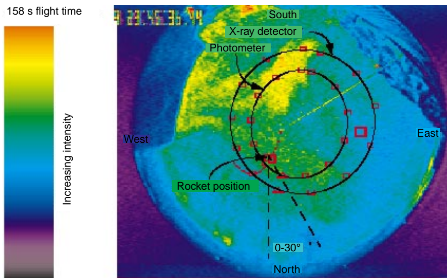
Fig. 3. All-sky TV picture at 158-s flight time. Projections down to the horizontal production layer are indicated for the scanning paths of the X-ray detector and the photometers, and down along the field line for the rocket position. The yellow streak in SE is produced by a lidar beam. The small red squares are the centre field of view at each centre time of data accumulation for the photometer and the X-ray detector. The large red square indicates the location of EISCAT
