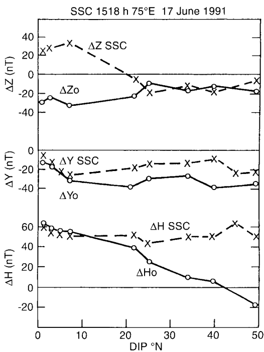
Fig. 7. Latitudinal variations in the amplitudes of SSC ( \Delta H_{SSC} , \Delta Y_{SSC} , and \Delta Z_{SSC} ) at 1518 h 75° EMT on 17 June 1991 and pre-SSC ( \Delta H_0 , \Delta Y_0 and \Delta Z_0 ) in the three components of the field
