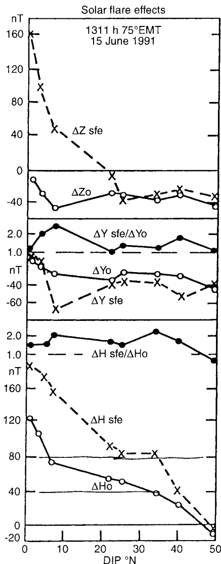
Fig. 4. Latitudinal variations in the amplitudes in the three components of the geomagnetic field during the flare ( \Delta Y_{SFE} , \Delta H_{SFE} and \Delta Z_{SFE} ) and pre-flare SQ ( \Delta Y_0 , \Delta H_0 and \Delta Z_0 ). Also the ratios of the amplitudes in Y and H components at SFE and pre-SFE times with latitudes are shown
