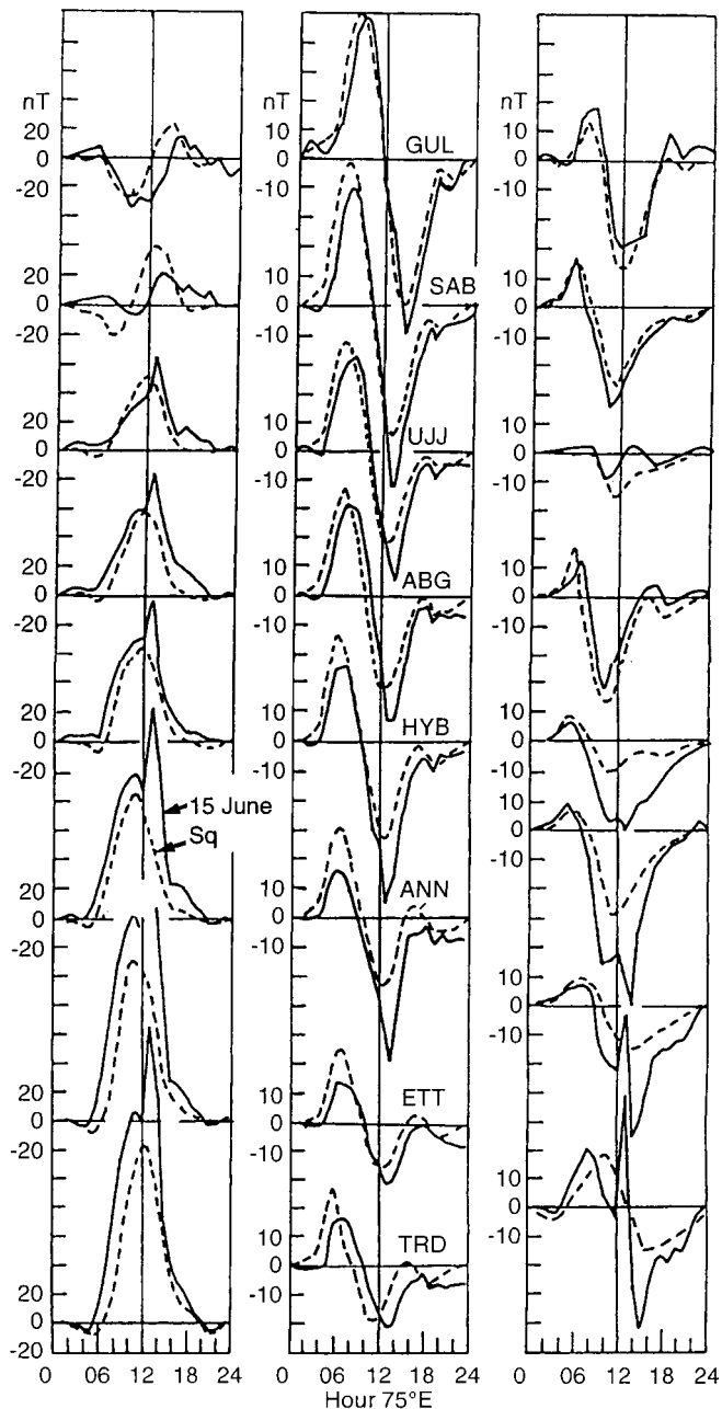
Fig. 2. The variations in the geomagnetic field H (left panel), Y (middle panel) and Z (right panel) at the Indian observatories averaged on five international quiet days of June 1991 ( dashed lines ); individual day 15 June 1991 ( full lines ). All curves constructed from hourly mean values
