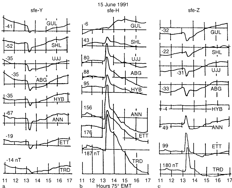
Fig. 3a-c. The magnetogram tracings at Indian Observatories showing the SFEs on a Y , b H and c Z components due to the flare at 1311 h 75° EMT on 15 June 1991. The amplitudes of SFE at each of the stations for the three components of geomagnetic field are indicated
