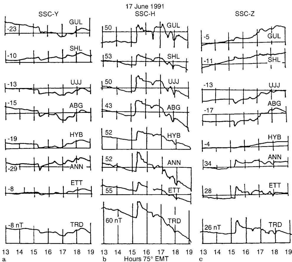
Fig. 6. Magnetogram tracings from Indian Observatories showing signatures of storm sudden commencement (SSC) at 1518 h 75° EMT on 17 June 1991. The amplitudes of SSC at each of the stations for the three components of the geomagnetic field in nT are indicated
