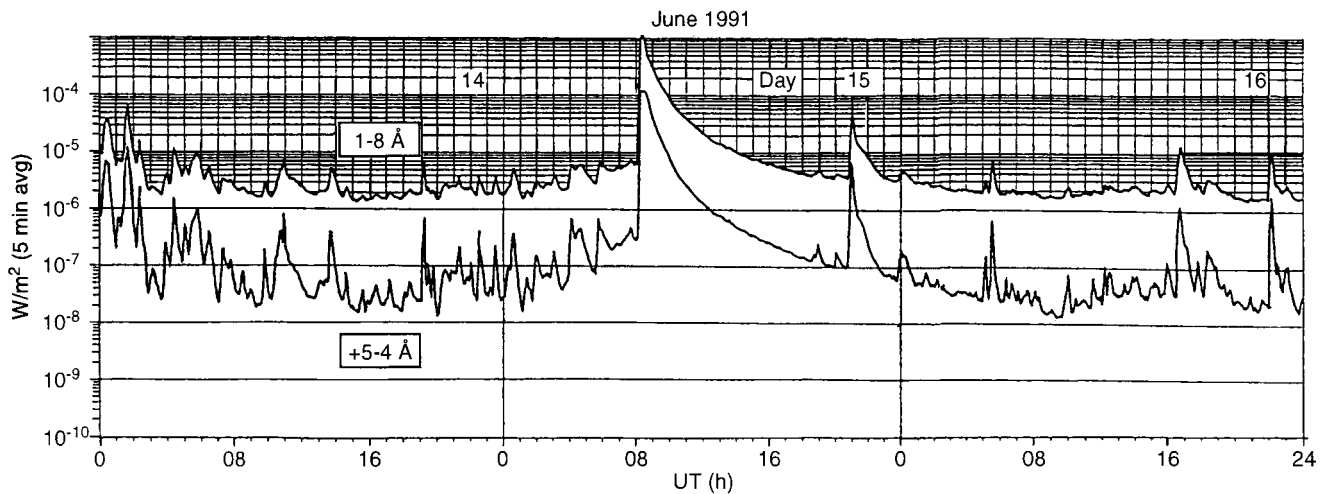
Fig. 1. Variation in solar X-ray flux within 0.5–4 and 1–8 Å ranges during 14–16 June 1991 by instruments aboard the GOES satellite
