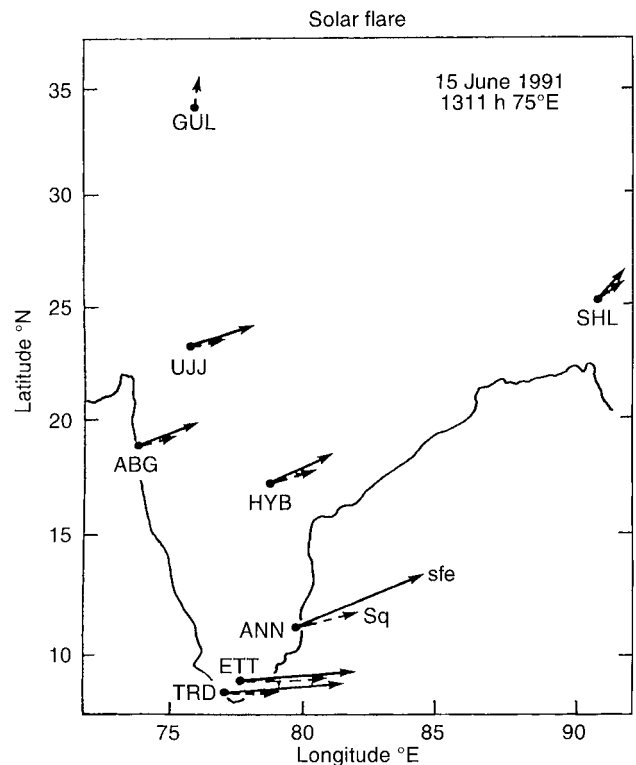
Fig. 5. Equivalent ionospheric current vectors (1) solar flare effect (continuous line) and (2) pre-flare SQ (dashed line), at Indian observatories
