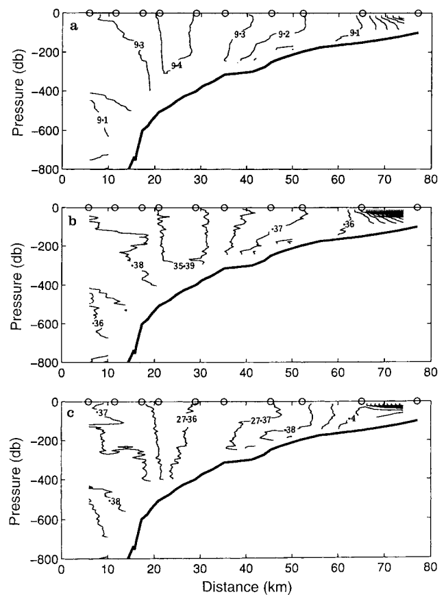
Fig. 3a-c. Vertical sections of a Potential temperature, b salinity and c \sigma_t , for the CTD transect shown in Fig. 1. Contour intervals are (a) 0.1^\circ\text{C} , (b) 0.01 and (c) 0.01\text{ kg m}^{-3} . Station positions are indicated by the open circles
