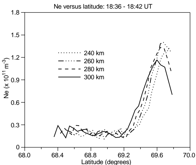
Fig. 3. Electron densities as a function of latitude for four selected heights measured by the radar during the scan commencing at 1836 UT
