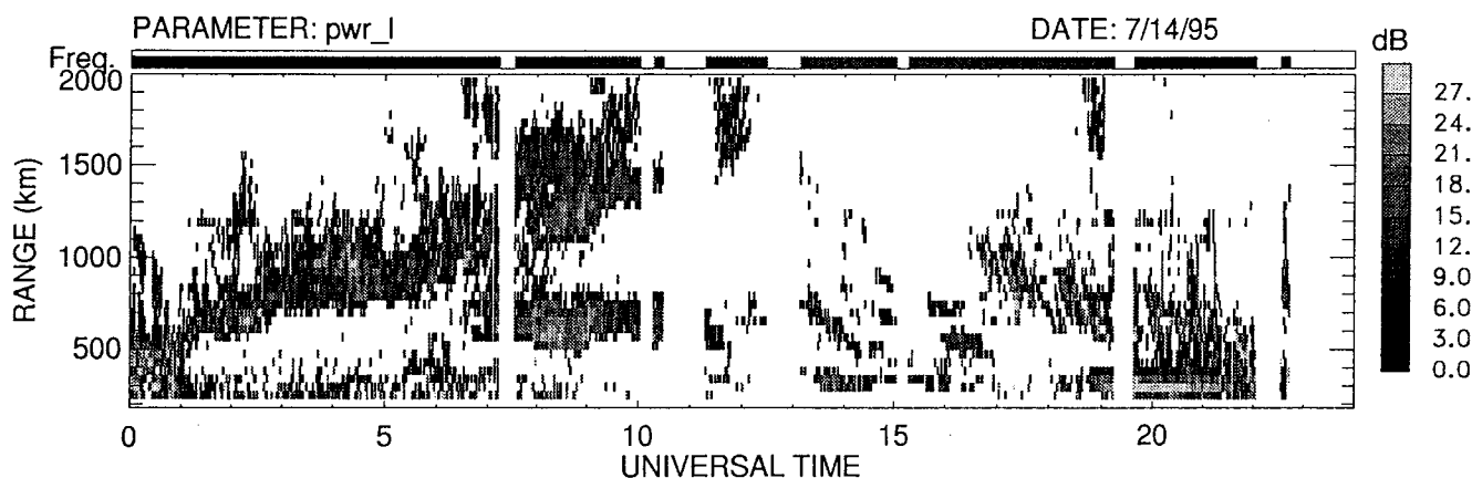
Fig. 7. Range-time-intensity plot of echo power observed on beam number 15 of Syowa Station HF radar on 14 July 1995. Beam 15 is directed toward the south magnetic pole (see Fig. 6). Radar frequen-
