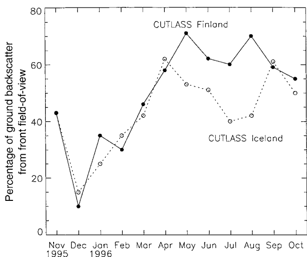
Fig. 8. The monthly variation in the percentage of ground backscatter originating in the front fields-of-view of the CUTLASS radars
