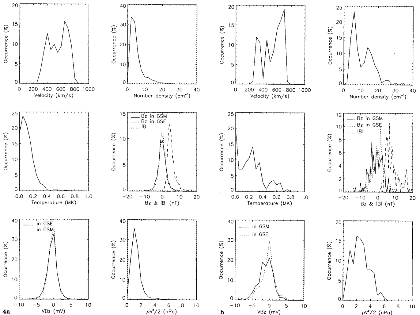
Fig. 4. a Distribution of solar-wind parameters in all the observed data. b Distribution of solar-wind parameters in the HSRs. c Distribution of solar-wind parameters in the CIRs
