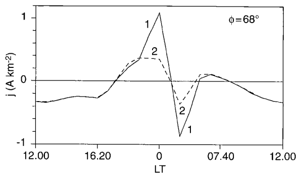
Fig. 4. The calculated longitudinal variations of the field-aligned current density along the 68^\circ geomagnetic latitude in the end of the substorm expansion phase for the cases: 1, the region of decreased magnetospheric conductivity is travelling westwards and 2, it is at rest
