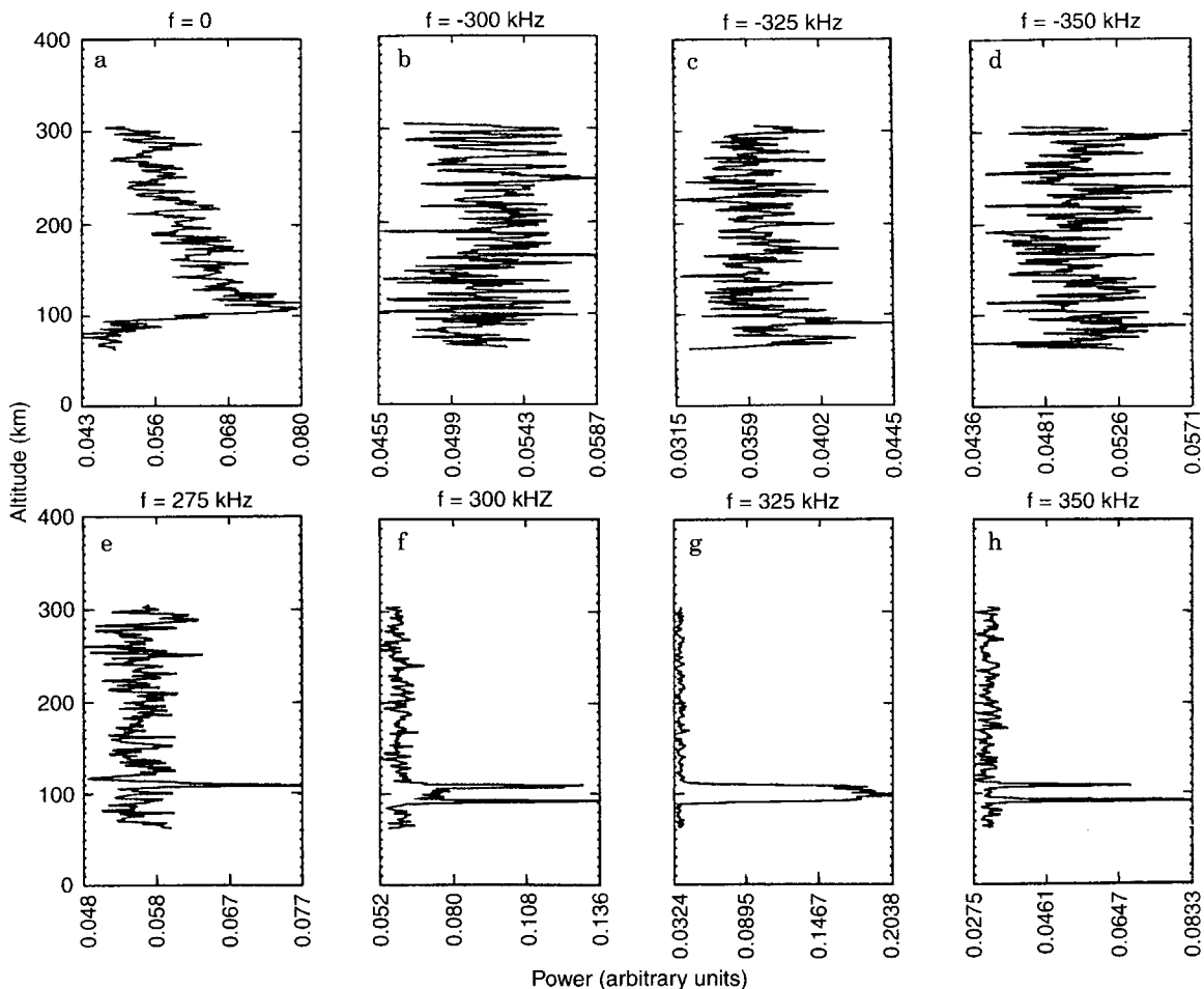
Fig. 7a–h. Power profiles between 1500:00 and 1500:10 UT on 17 August 1993 for Az = 0^\circ and EI = 20^\circ . a ion-line profile; b–d downshifted receiver channels at f = -300 , -325 and
