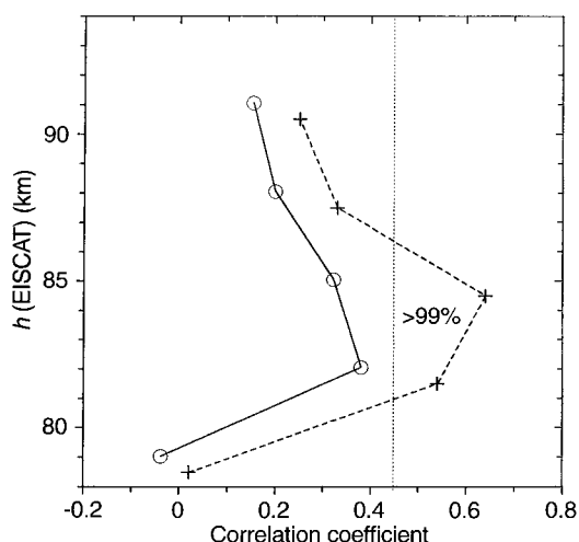
Fig. 9. Correlation between hourly SNR values deduced from EISCAT VHF and MF-radar observations as a function of height using SNR values at equal heights ( solid line ) and at different heights ( dashed line : h(\text{EISCAT}) = h(\text{MF}) + 2.5 \text{ km} )
