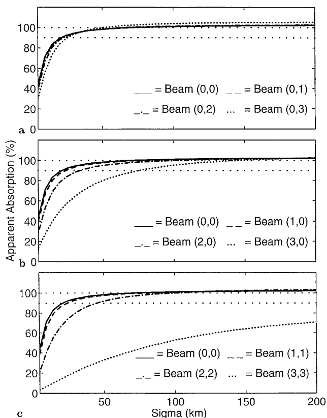
Fig. 14a–c. Ratio of apparent-to-true zenithal absorption for an E-W absorption strip observed with selected beams of a 49-beam IRIS. The strip is of Gaussian form in the N-S direction and its maximum absorption is 3 dB in each case. (the results would be slightly different for other maximum values); the 90% level is indicated. a Beams to the east; b beams to the north; c beams to the north-east
